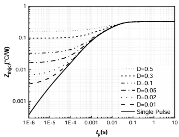
Fig 8 Transient Thermal Impandance
