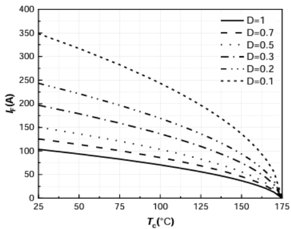
Fig 5 Current Derating
